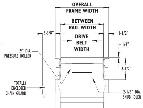
SECTION "X-X"
